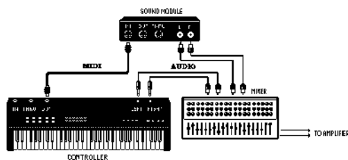
Signal paths for external MIDI instruments
