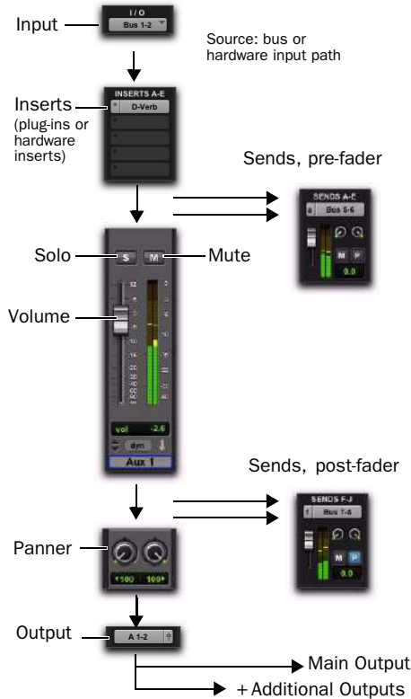
Auxiliary Input track audio signal flow
