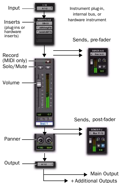
Instrument track audio signal flow
